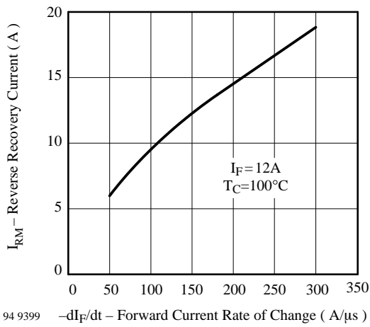
Figure 9 : Reverse Recovery Current vs. Forward Current Rate of Change
